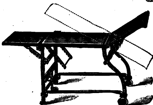
S.P. 927. Bailey's "Simplex" Operation Table. A perfectly rigid table, giving a good Trendelenburg position. Lever action and third wheel and leg crutches. £11 10 0
