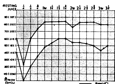
Superimposed gruel fractional test-meal curve of five cases of duodenal ulcer.
