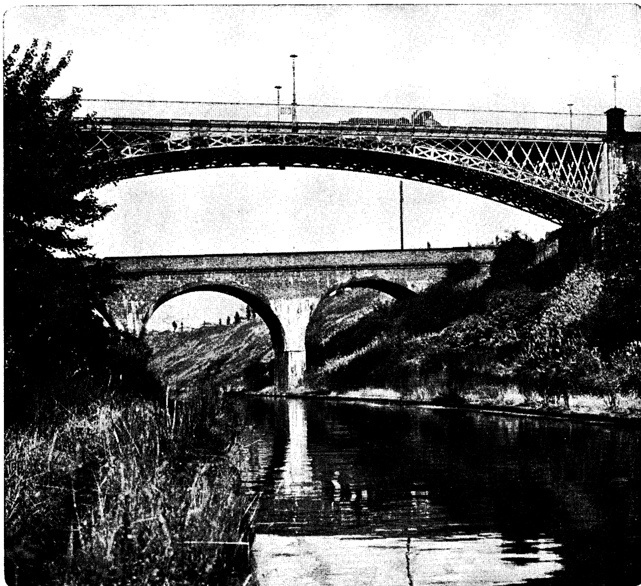
The cast-iron Gallton Bridge at Smethwick was designed by Thomas Telford, and built in 1829. It carries the road over the Birmingham Canal.
