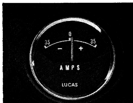
Ammeter plus the new high-charge alternator – ensures your battery stays in peak condition.
