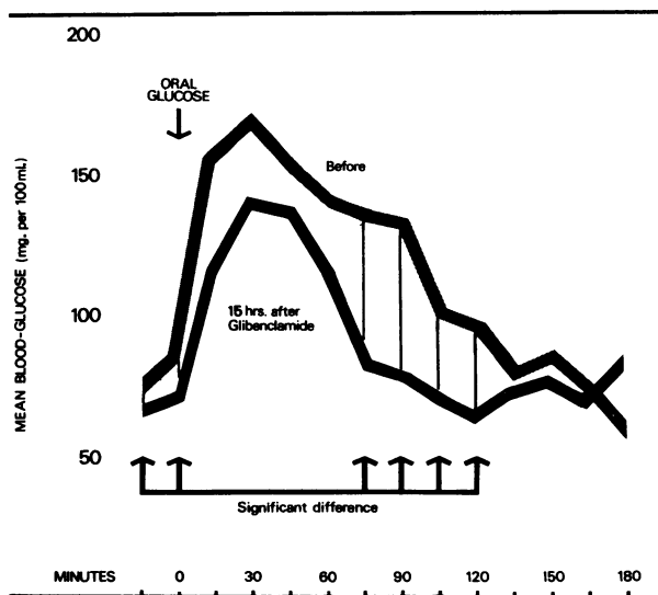
Effect of an oral glucose load on mean blood-glucose in four healthy adults before and 15 hours after 5 mg. glibenclamide.
