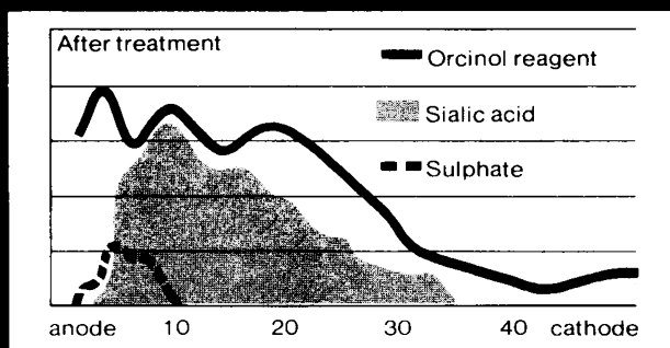
Same patient after 10 days' treatment with Mucodyne — proportion of sialomucins is greatly increased.
