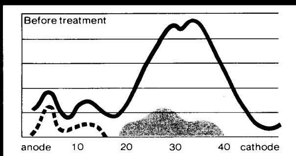
Electrophoretic pattern of mucus typical of chronic bronchitis — sialomucin content is low.
