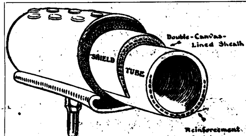
The Victor Combination Tube and Sheath. SAVES 50% TYRE COST
