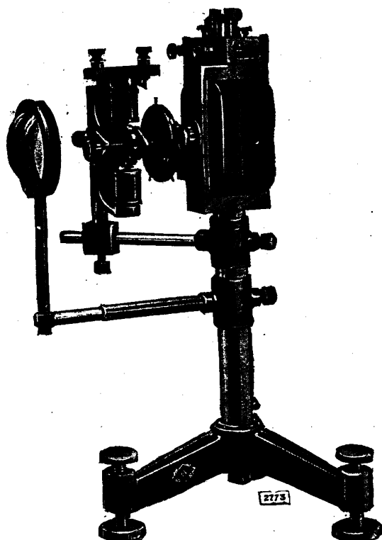
Cambridge Small String Galvanometer on stand, with Time-marking apparatus and cylindrical lens.
