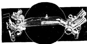
A typical 'K' type tilt-starting quartz burner, about 1/5 real scale.
