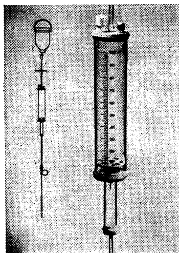
METRASET (measured volume solution administrative set) McGAW No. 2021
