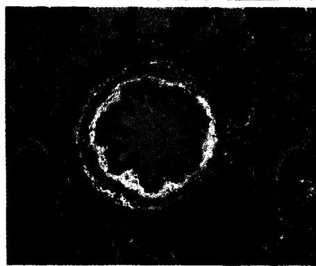
Cross section of a bronchiole showing BRONCHIAL MUCOSAL OEDEMA
