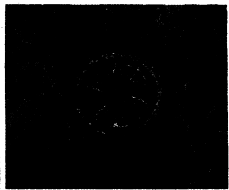
Cross section of a bronchiole showing BRONCHOSPASM
