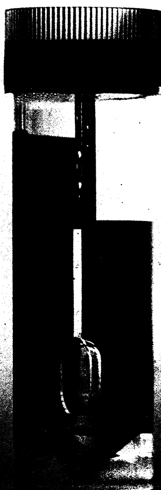
Klebsiella aerogenes
